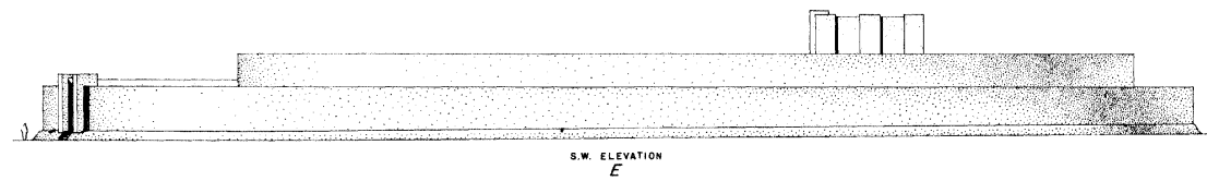
RECONSTRUCTED ELEVATIONS AND CROSS SECTIONS OF THE TEMPLE OVAL OF THE FIRST BUILDING PERIOD. SCALE, 1:450
